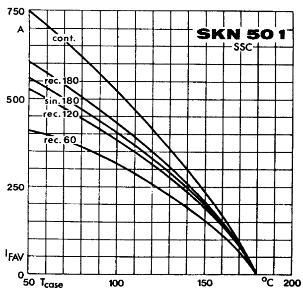
Fig. 3 d Rated forward current vs. case temperature
