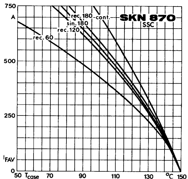
Fig. 3 f Rated forward current vs. case temperature
