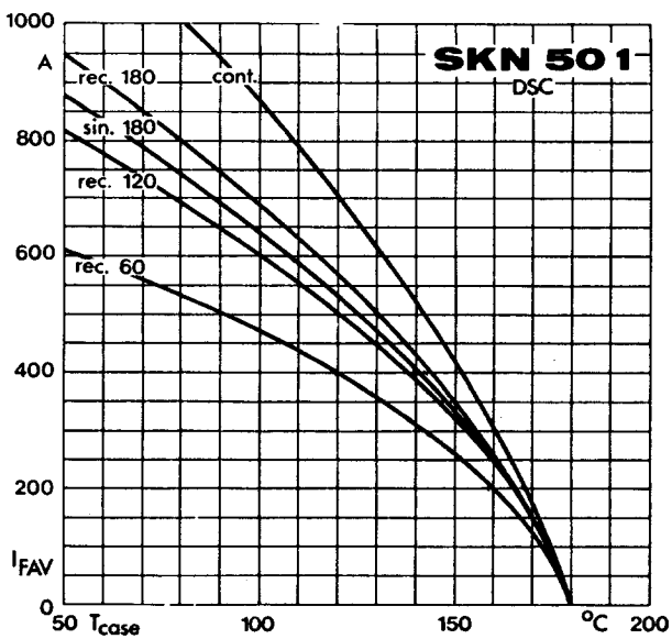
Fig. 3 c Rated forward current vs. case temperature
