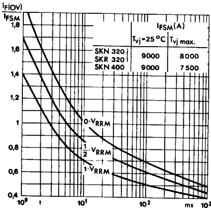
Fig. 7 Surge overload current vs. time
