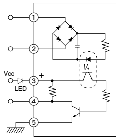
1) AC input module Without LED With LED
