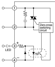
3) AC output module Without LED With LED
