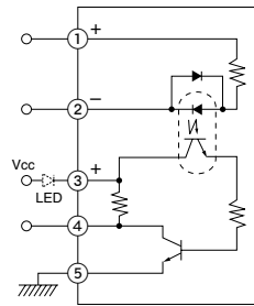
2) DC input module Without LED With LED
