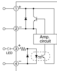
4) DC output module Without LED With LED
