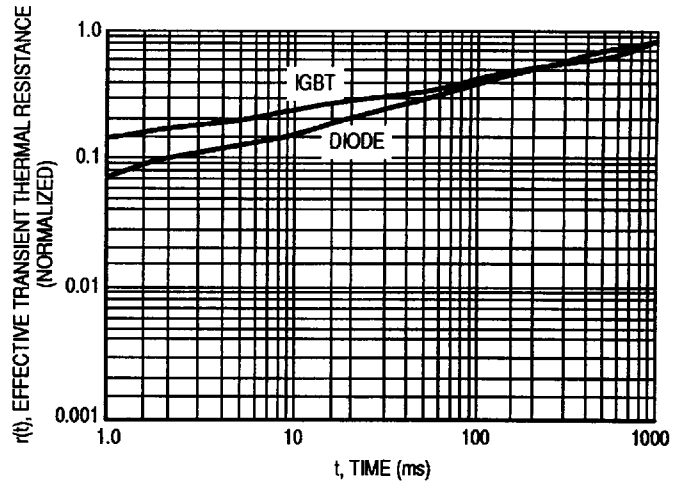
Figure 18. Thermal Response
