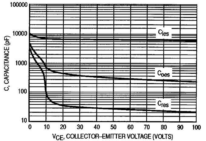
Figure 16. Capacitance Variation
