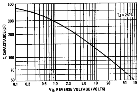
FIGURE 7 - CAPACITANCE
