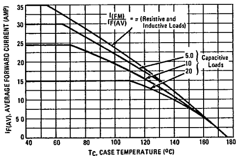
FIGURE 4 - CURRENT DERATING
