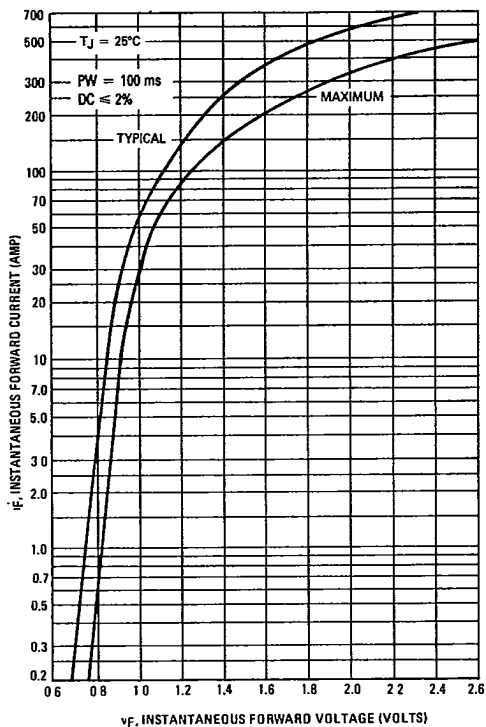
FIGURE 1 - FORWARD VOLTAGE
