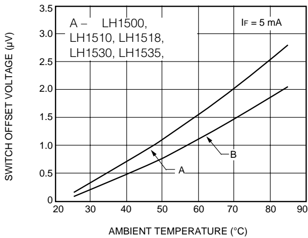
E. Switch Offset Voltage vs. Temperature
