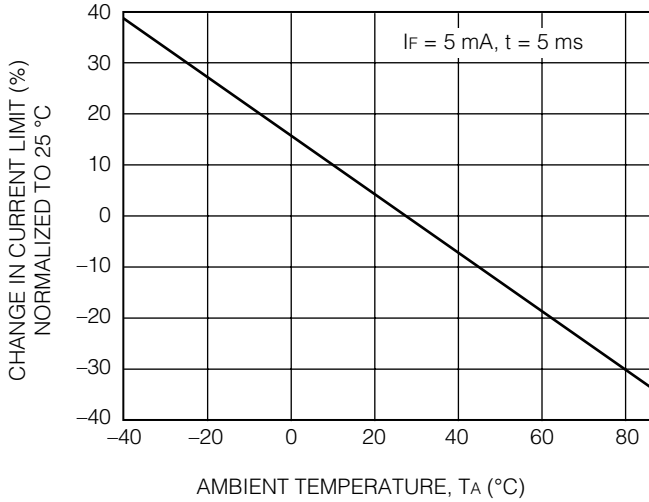
C. Current Limit vs. Temperature
