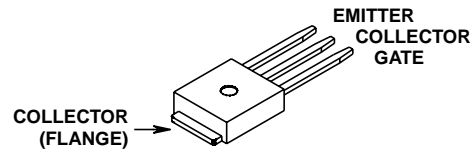
HGTD10N40F1, HGTD10N50F1 JEDEC TO-251AA
