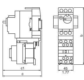
Combination GV2P + TeSys D range contactor
