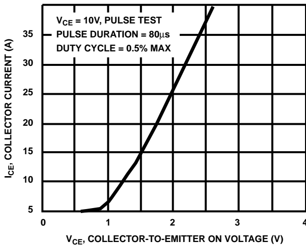
FIGURE 5. TYPICAL COLLECTOR-TO-EMITTER ON-VOLTAGE vs COLLECTOR CURRENT
