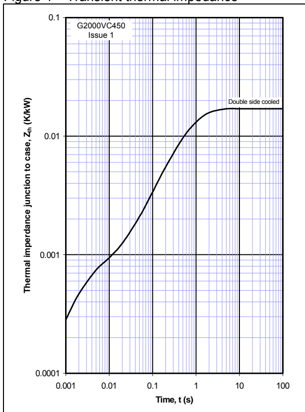
Figure 4 – Transient thermal impedance
