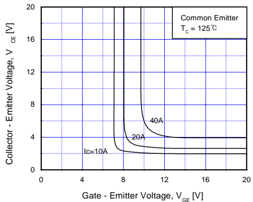
Fig 6. Saturation Voltage vs. V_{GE}
