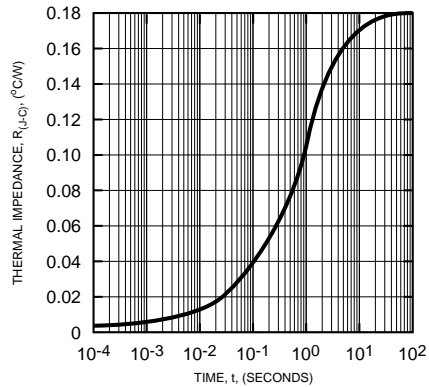
MAXIMUM TRANSIENT THERMAL IMPEDANCE (JUNCTION-TO-CASE) (PER SCR)
