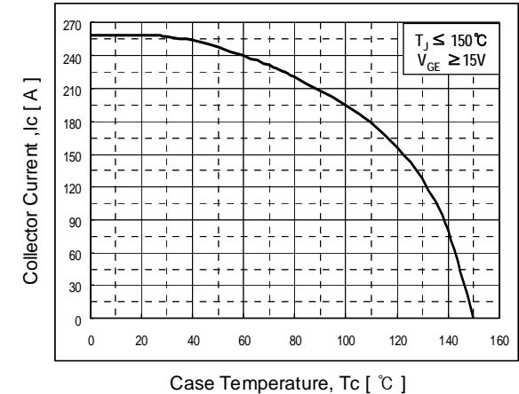
Fig 12. rated Current vs. Case Temperature
