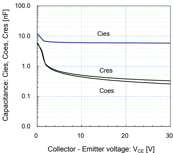
[ Inverter ] Capacitance vs. Collector-Emittter voltage (typ.) VGE=0V, f= 1MHz, Tj= 25°C
