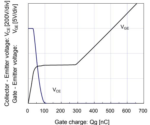
[ Inverter ] Dynamic gate charge (typ.) Vcc=600V, Ic=75A, Tj= 25°C
