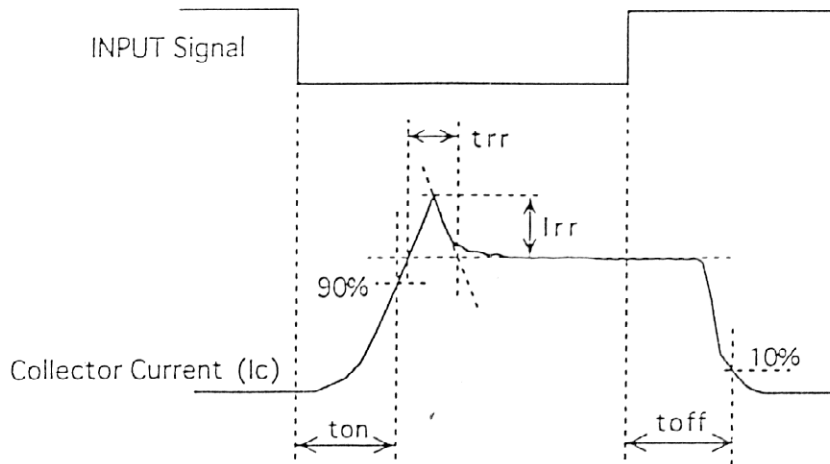
Fig.4 : Definition of switching time
