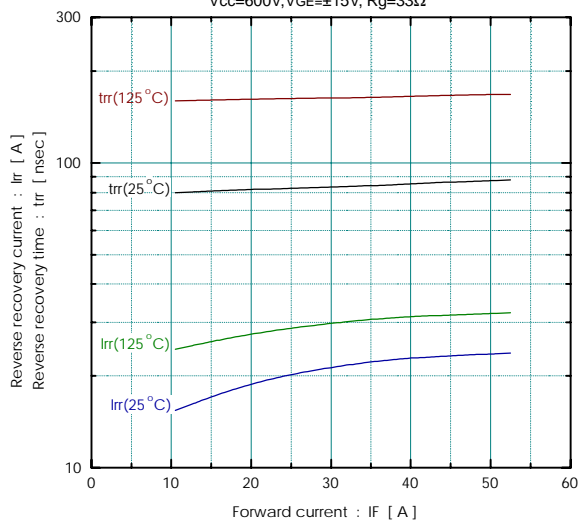
Reverse recovery characteristics (typ.) Vcc=600V, VGE=±15V, Rg=33Ω
