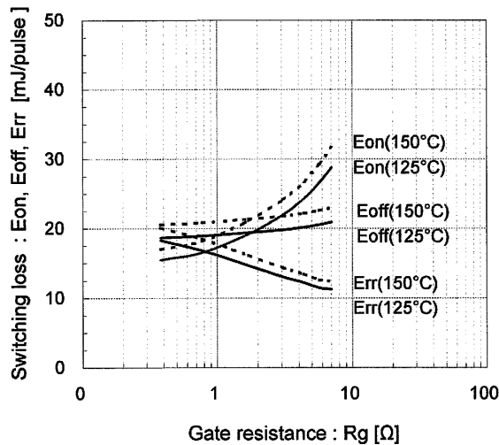
Switching loss vs. gate resistance (typ.) V_{CC}=600V, I_c=200A, V_{GE}=\pm 15V
