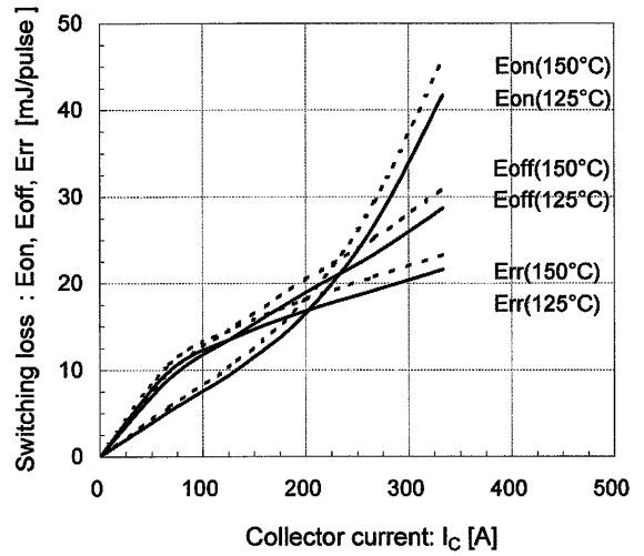
Switching loss vs. Collector current (typ.) V_{CC}=600V, V_{GE}=\pm 15V, R_g=1.2\Omega
