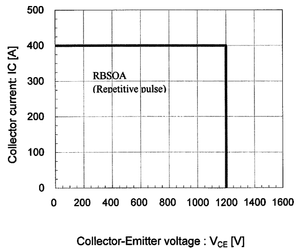
Reverse bias safe operating area (max.) +V_{GE}=15V, -V_{GE} \le 15V, R_g \ge 1.2\Omega, T_j \le 125^\circ C
