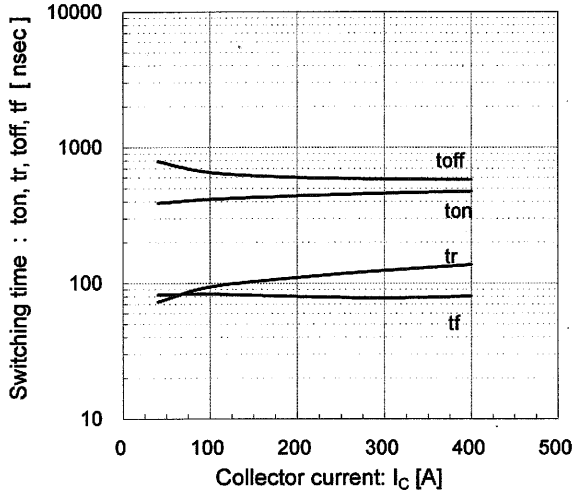
Switching time vs. Collector current (typ.) V_{CC}=600V, V_{GE}=\pm 15V, R_g=1.2\Omega, T_j=125^\circ C
