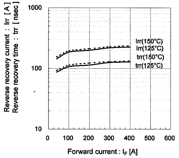
[ Inverter ] Reverse recovery characteristics (typ.) V_{CC}=600\text{V} , V_{GE}=\pm 15\text{V} , R_g=1.2\Omega
